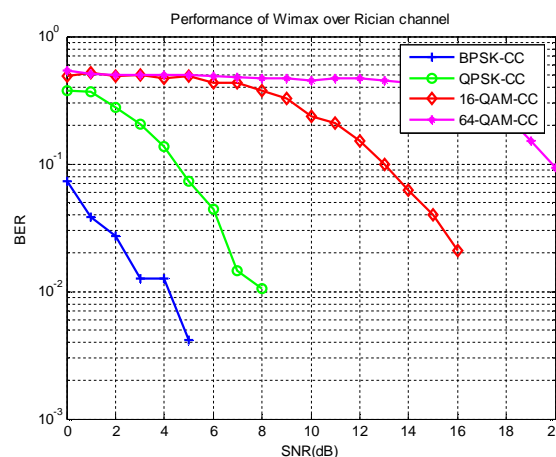
Fig.4: WiMAX performance in Rician for CC code
