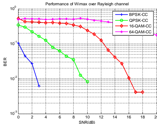
Fig.3: WiMAX performance in Rayleigh channel for CC code
