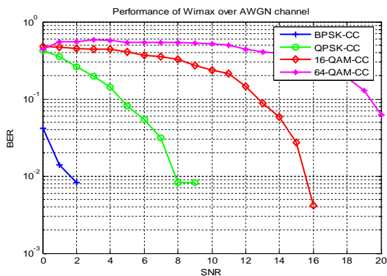
Fig.2: WiMAX performance in AWGN channel for CC code
