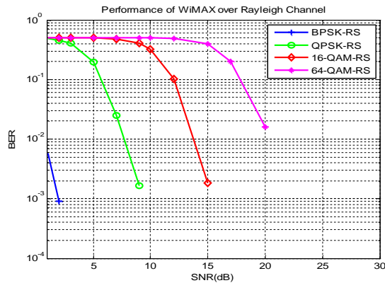
Fig.6: WiMAX performance in Rayleigh channel for RS code
