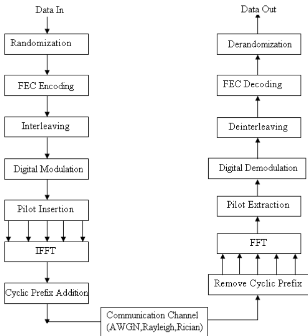
Fig.1: Block diagram of WiMAX WiMAX
