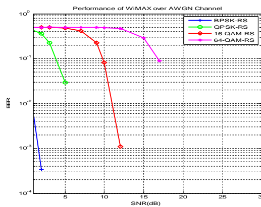
Fig.5: WiMAX performance in AWGN channel for RS code
